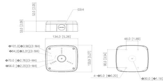
Dimensions (mm[inch])
